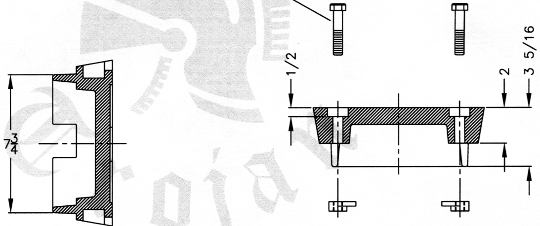
SECTION B-B
