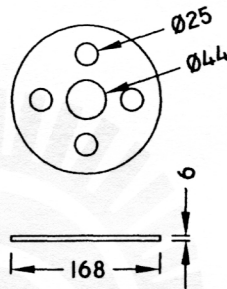
GUIDE PLATE
