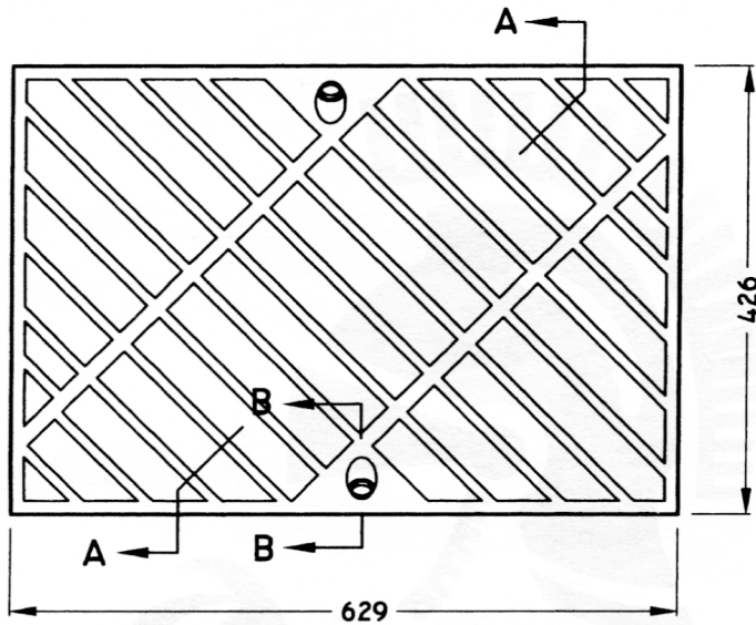
PLAN
