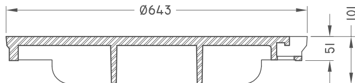
SECTION
