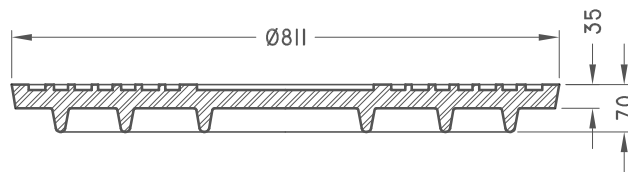
SECTION
