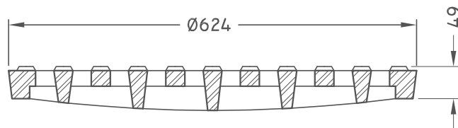
SECTION
