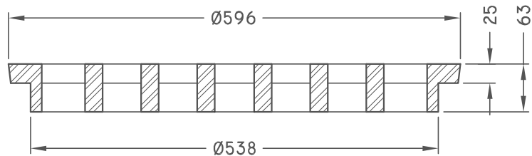
SECTION
